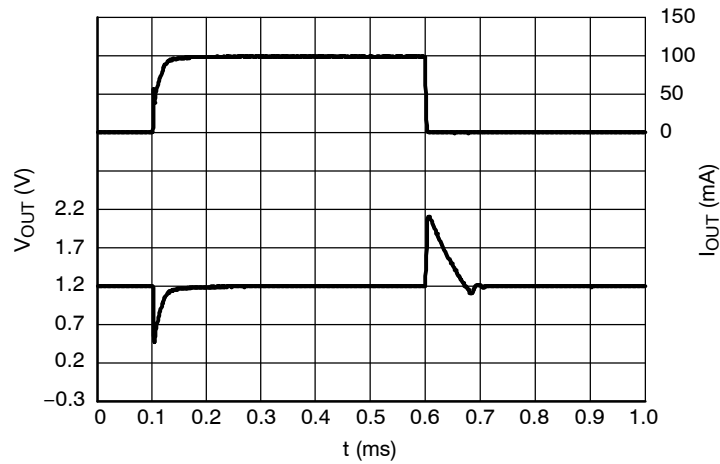
Figure 47. Load transients, 1.2 V Version, I OUT = 1 – 100 mA, t R = t F = 0.5 μs, V IN = 2.2 V
