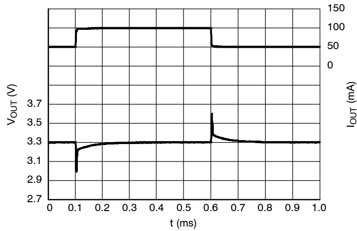
Figure 46. Load Transients, 3.3 V Version, I OUT = 50 – 100 mA, t R = t F = 0.5 μs, V IN = 4.3 V
