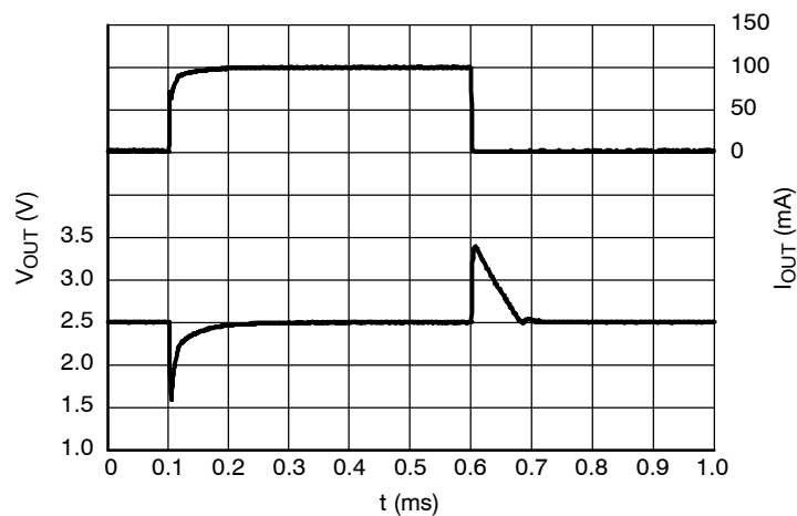
Figure 48. Load Transients, 2.5 V Version, I OUT = 1 – 100 mA, t R = t F = 0.5 μs, V IN = 3.5 V
