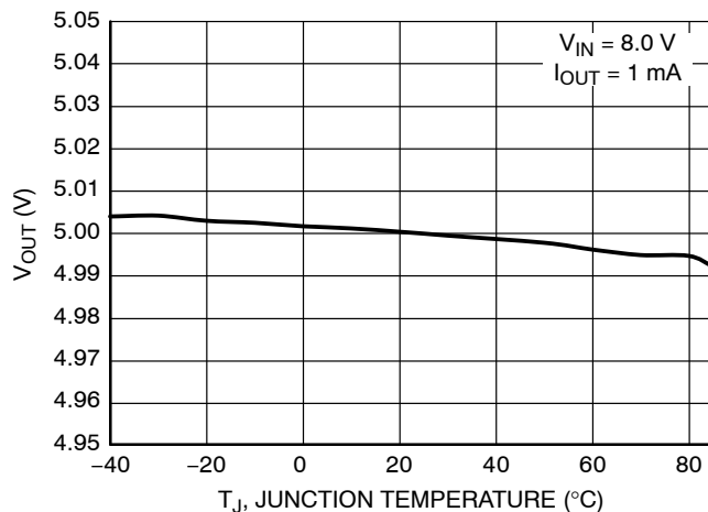
Figure 20. Output Voltage vs. Temperature, 5.0 V Version, ECO = H
