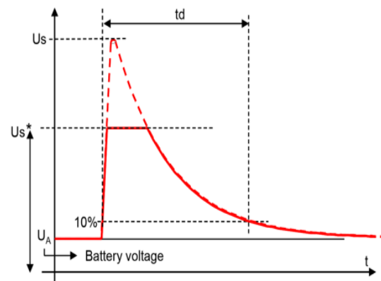
Figure 20. ISO16750-2 test B definition
