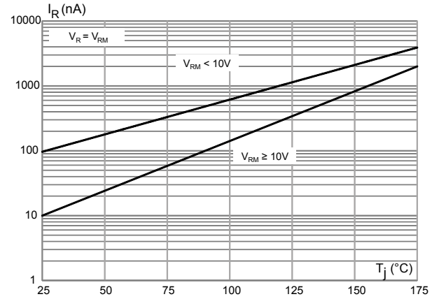
Figure 8. Leakage current versus junction temperature
