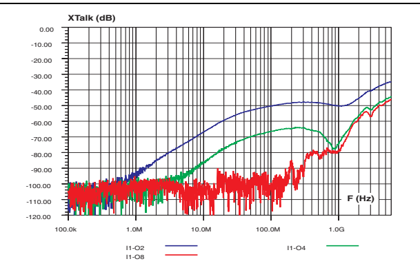
Figure 5. Analog crosstalk measurements
