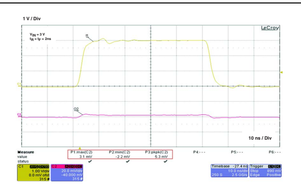
Figure 9. Typical digital crosstalk
