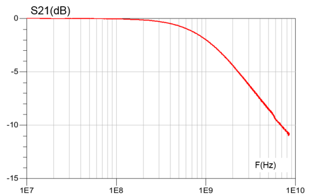
Figure 7. S21 attenuation
