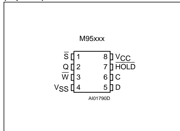
Figure 3. 8-pin Package Connections (Top View)
