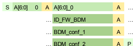
Figure 18. Without parity detection (4 bytes)
