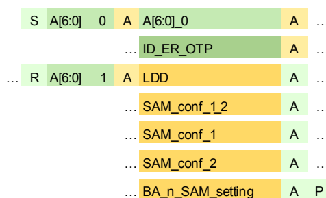
Figure 42. Read back OTP bit without parity detection
