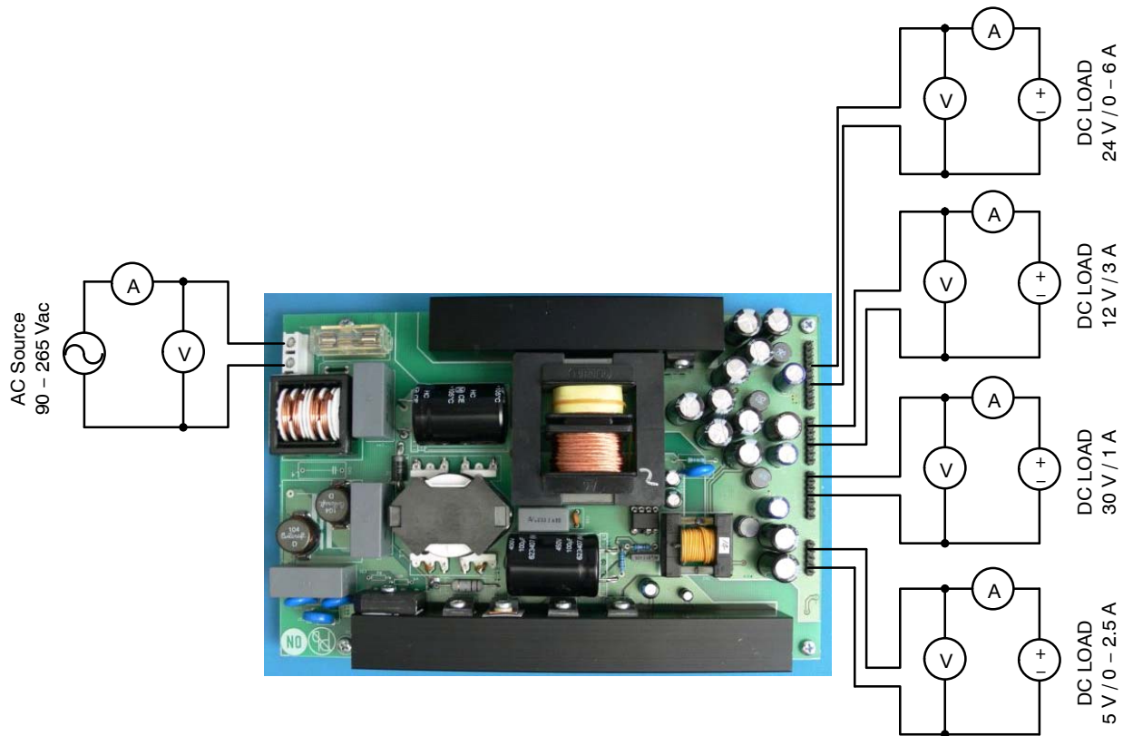
Figure 25. Test Setup
