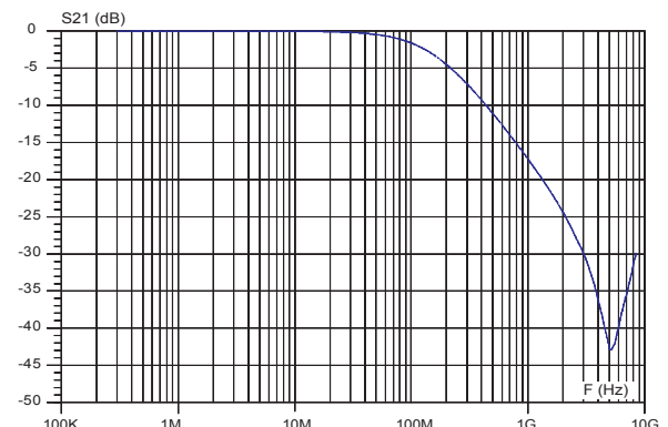
Figure 7. S21 attenuation
