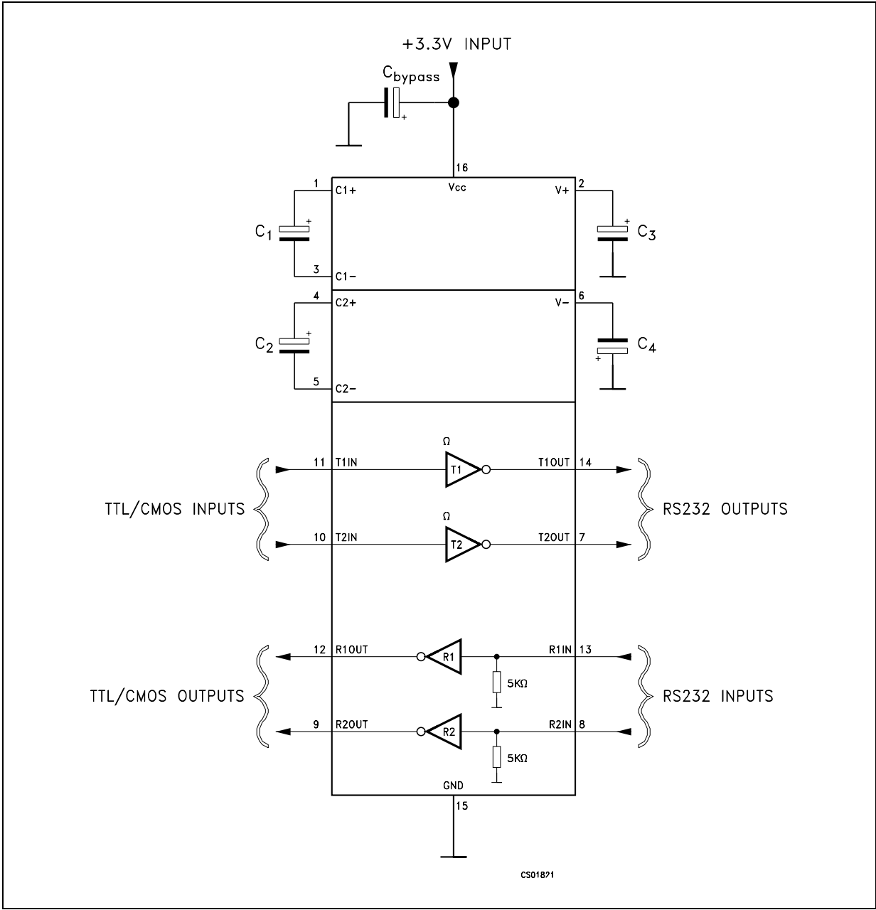
Figure 3. Application circuits
