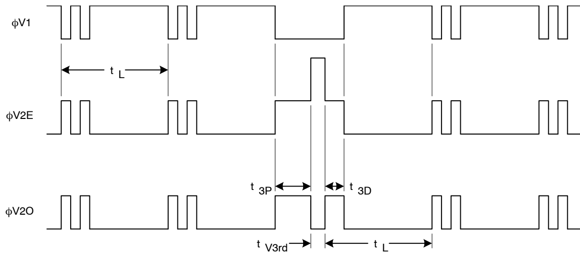
Figure 16. Interlaced Frame Timing – Frame Integration Mode – Even Field Readout
