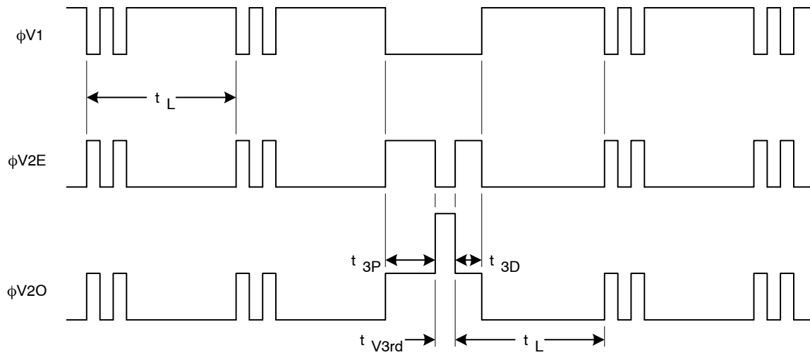
Figure 17. Interlaced Frame Timing – Frame Integration Mode – Odd Field Readout
