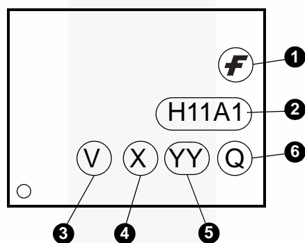
Figure 15. Top Mark
