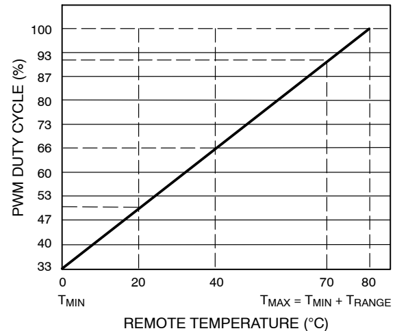
Figure 25. Max Speed Calculated by Remote Temperature Control Loop Drives Fan
