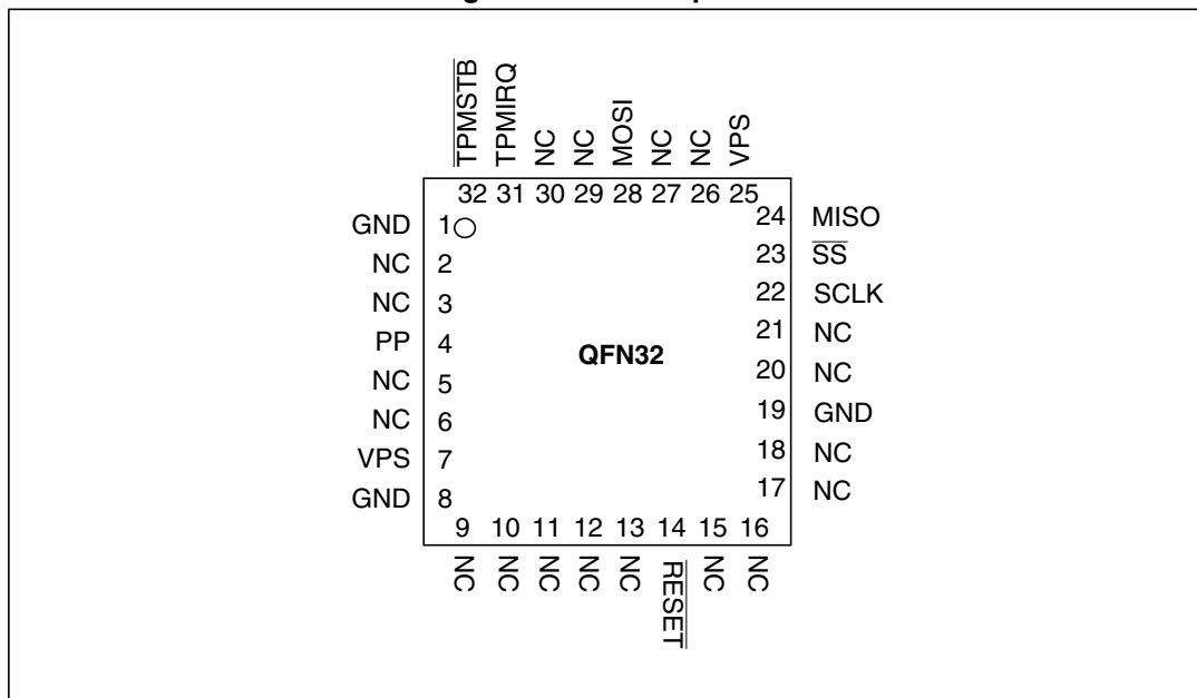
Figure 3. VQFN32 pinout
