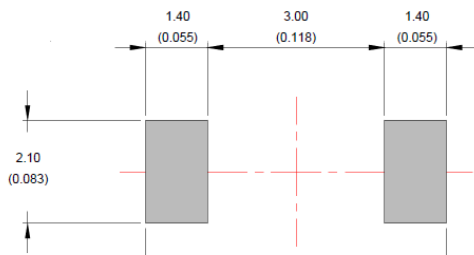
Figure 17. Footprint recommendations, dimensions in mm (inches)
