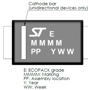
Figure 18. Marking layout (refer to ordering information table for marking)
