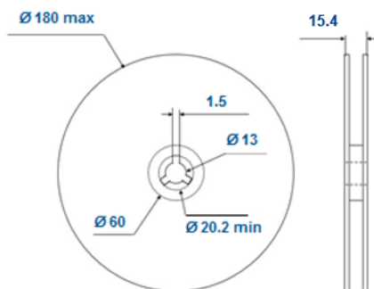
Figure 21. Reel dimensions (mm)
