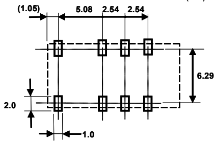
NOTE. General tolerance : \pm 0.1 (Top view)
