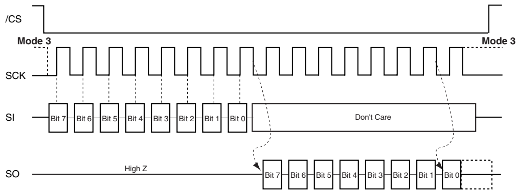
FIGURE 2. SPI Protocol
