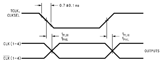
FIGURE 2. Propagation Delay, TCLK, CLKSEL to Outputs
