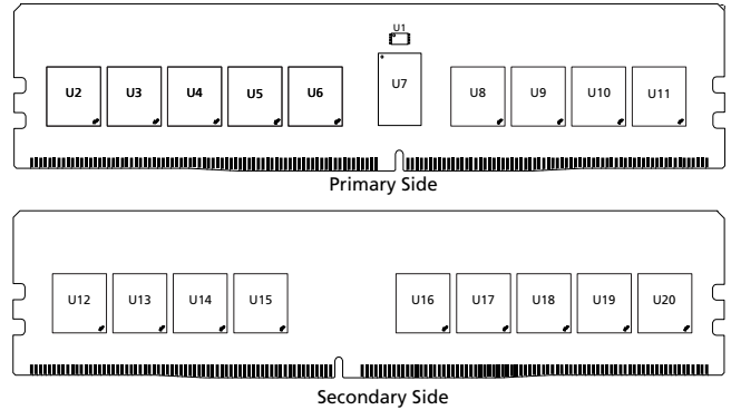
Figure 1: 288-Pin RDIMM (R/C-E3)
