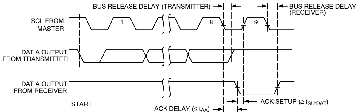
Figure 7. Acknowledge Timing
