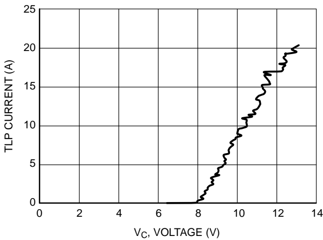
Figure 6. Positive TLP I-V Curve (Preliminary)
