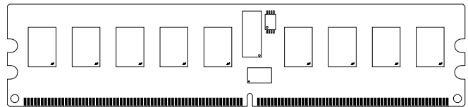
Figure 1: 240-Pin RDIMM (MO-237 R/C G)
