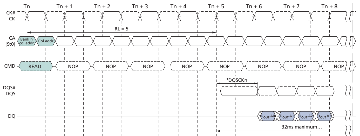
Figure 33: t_{DQSKDL} Timing
