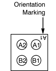
CM1230-02/J2 4-bump CSP Package
