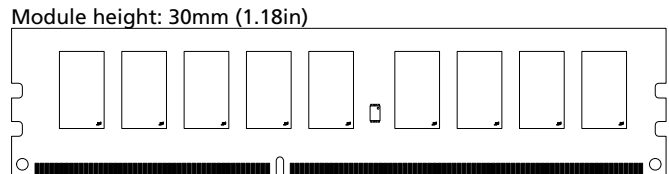
Figure 1: 240-Pin UDIMM (MO-269 R/C E)
