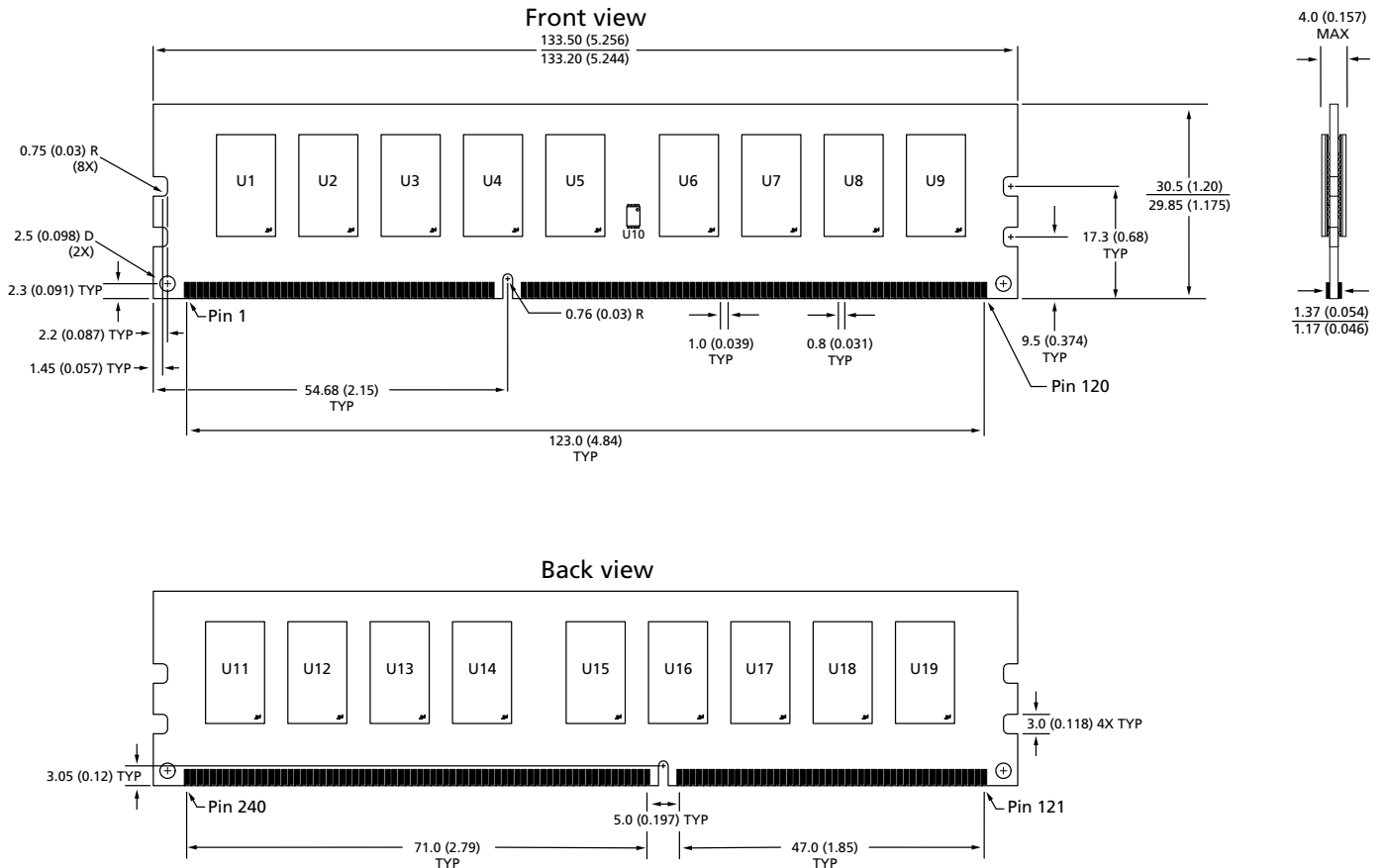
Figure 3: 240-Pin DDR3 UDIMM
