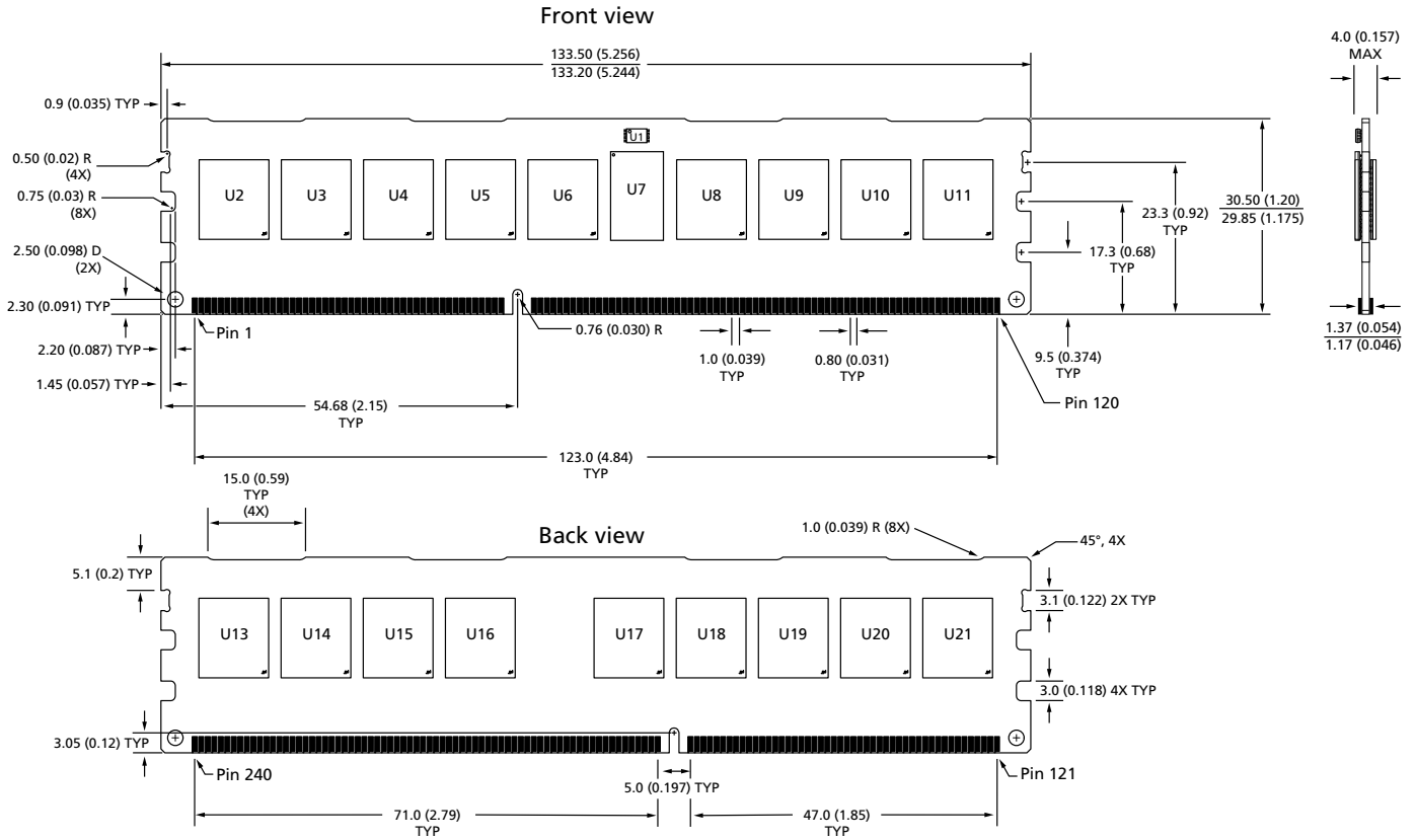
Figure 4: 240-Pin DDR3 RDIMM (PCB 1164)
