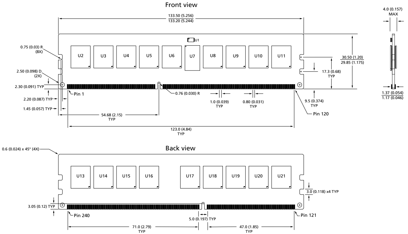
Figure 5: 240-Pin DDR3 RDIMM (PCB 1560)
