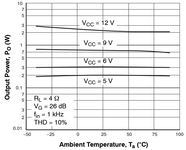
Figure 42. P_O - T_a
