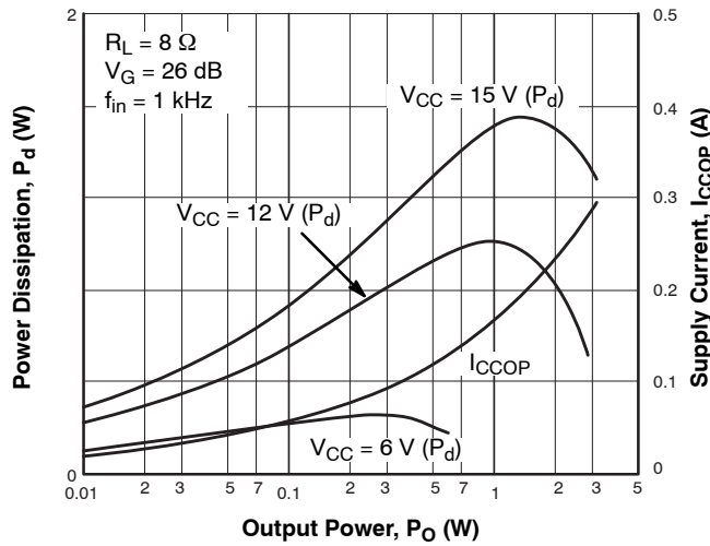
Figure 24. P_d - P_O
