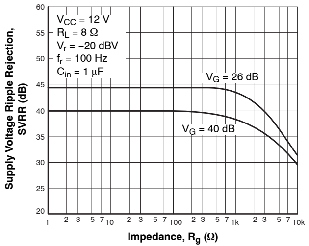
Figure 29. SVRR – R_g
