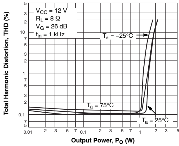
Figure 39. THD - P_O
