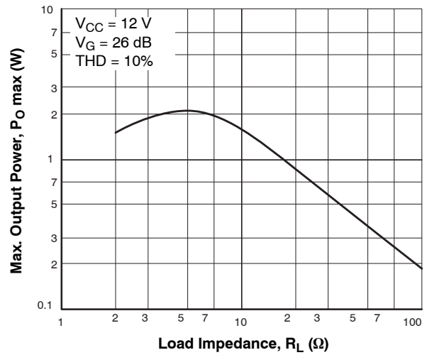
Figure 31. P_O max – R_L
