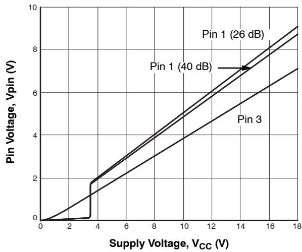
Figure 34. V_{pin} - V_{CC}
