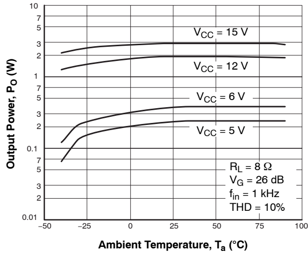
Figure 41. P_O - T_a
