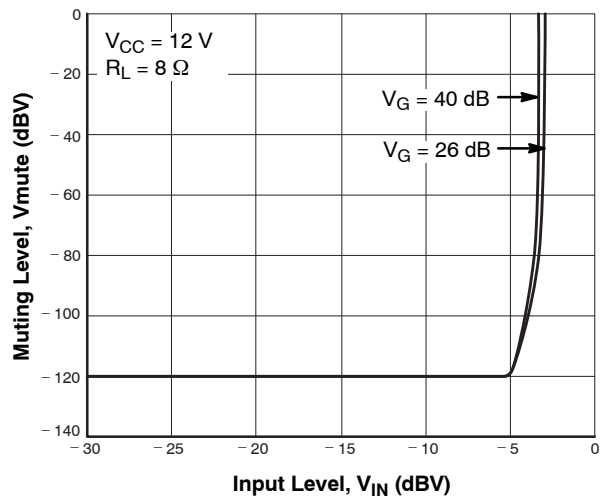
Figure 33. V_{mute} – V_{IN}
