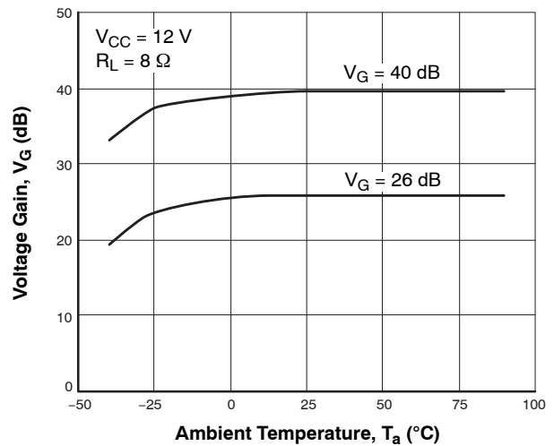
Figure 44. V_G - T_a
