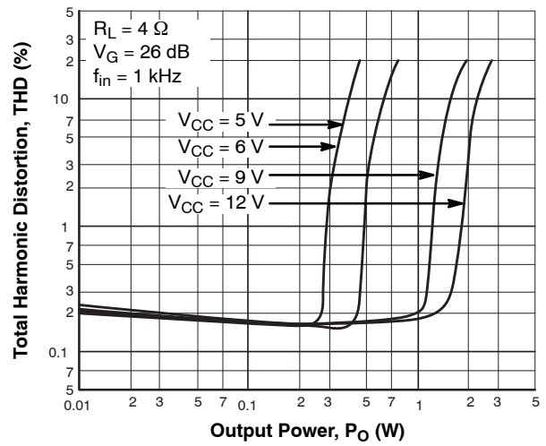
Figure 17. THD – P_O
