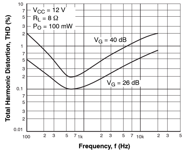
Figure 19. THD – f
