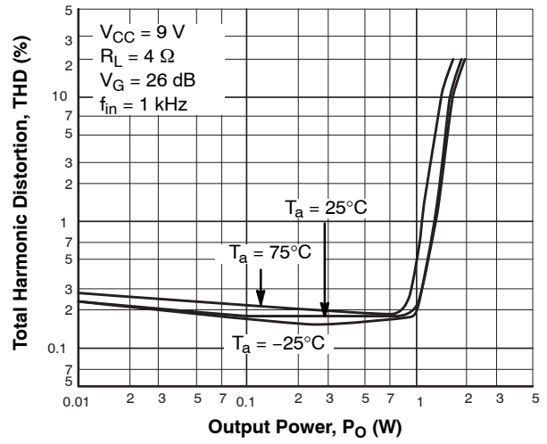
Figure 40. THD - P_O
