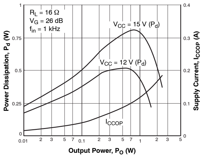
Figure 26. P_d - P_O
