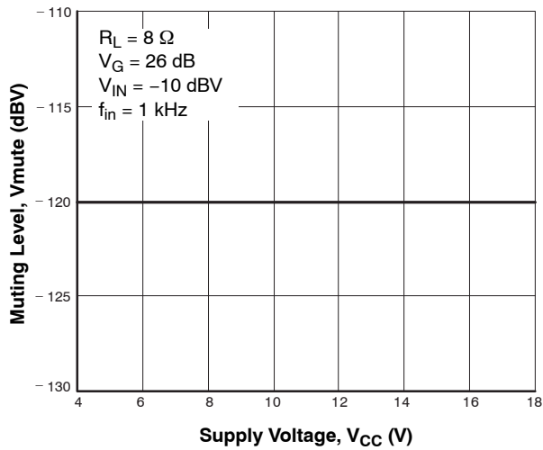
Figure 36. V_{mute} - V_{CC}
