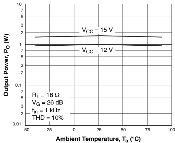
Figure 43. P_O - T_a
