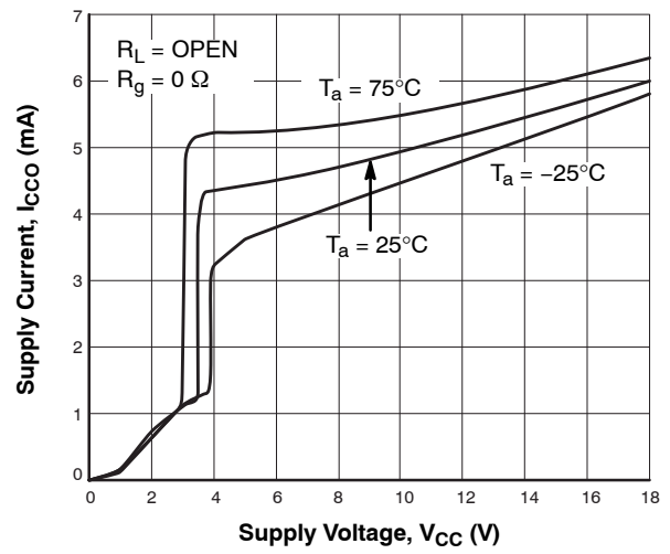
Figure 48. I_{CCO} - V_{CC}
