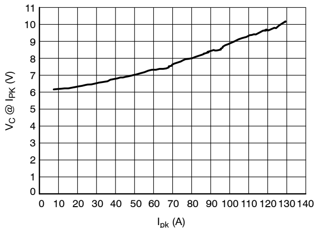
Figure 4. Clamping Voltage vs. Peak Pulse Current ( t_p = 8/20 \mu s )
