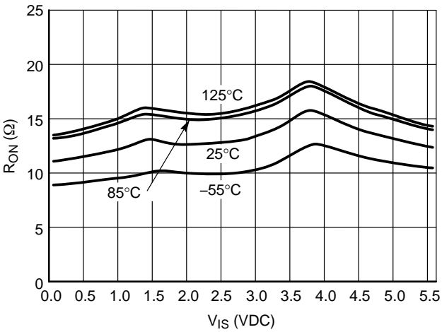
Figure 22. R_{ON} vs. Temp, V_{CC} = 5.5 V
