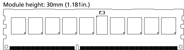
Figure 2: 240-Pin RDIMM (R/C B1)
