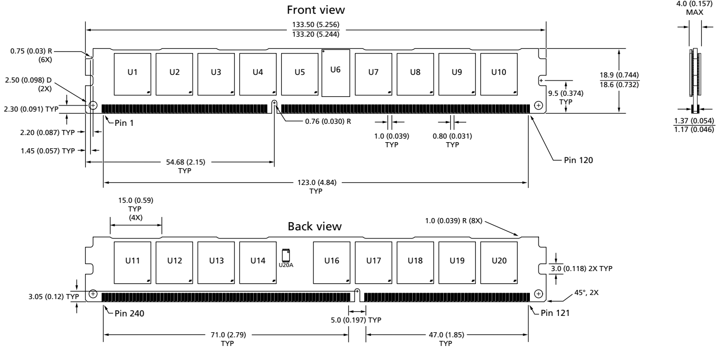
Figure 4: 240-Pin DDR3 RDIMM (R/C-L)
