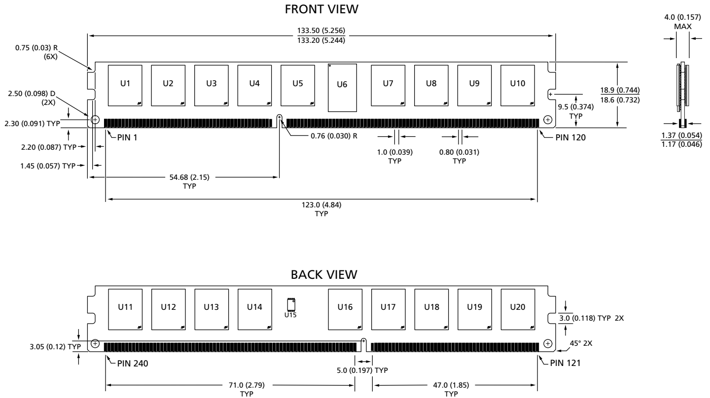
Figure 5: 240-Pin DDR3 RDIMM (R/C-L1)
