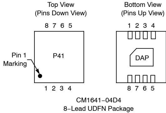
PACKAGE / PINOUT DIAGRAMS
