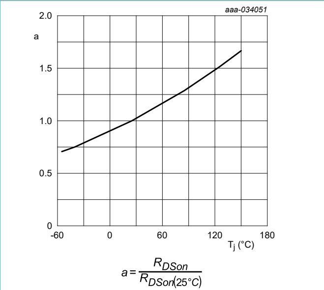
Fig. 11. Normalized drain-source on-state resistance as a function of junction temperature; typical values
