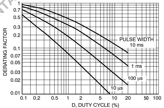
Figure 5. Typical Derating Factor for Duty Cycle
