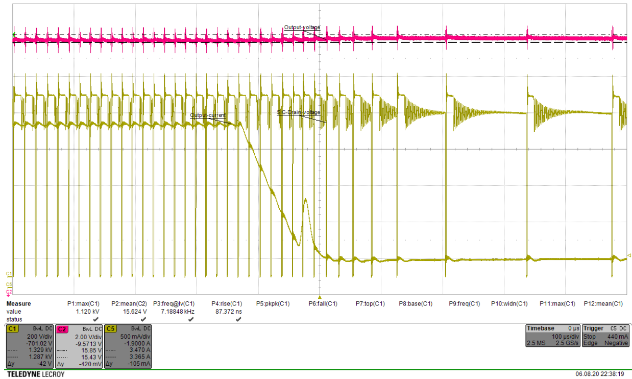
Figure 17. 900 V – 85% to 15%
