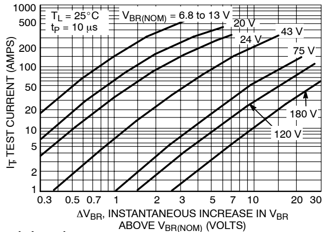
Figure 5. Dynamic Impedance
