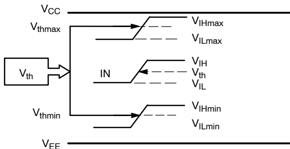
Figure 8. V th Diagram
