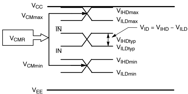
Figure 11. V CMR Diagram
