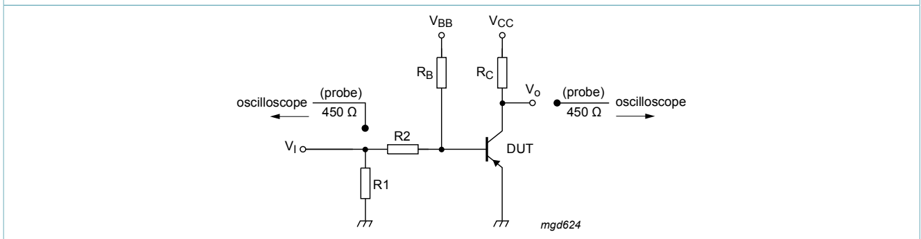
Fig. 15. Test circuit for switching times
