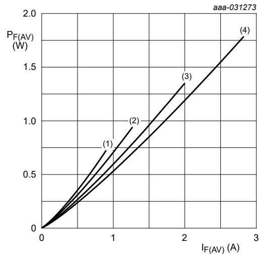
T_j = 175\text{ }^\circ\text{C} (1) \delta = 0.1 (2) \delta = 0.2 (3) \delta = 0.5 (4) \delta = 1 ; DC
