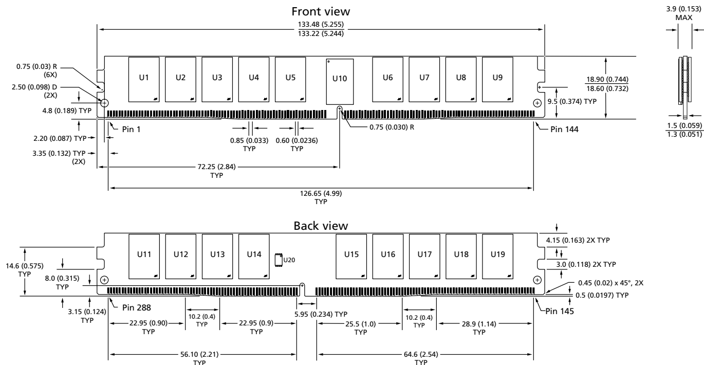
Figure 4: 288-Pin DDR4 VLP RDIMM (PCB 1714, 2463)
