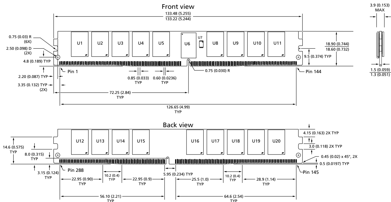
Figure 5: 288-Pin DDR4 VLP RDIMM (PCB 2954)
