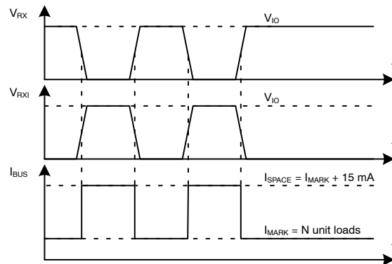
Figure 8. Output Waveforms
