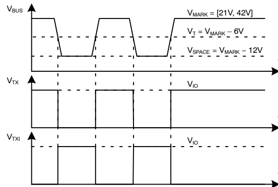
Figure 9. Receive Waveforms
