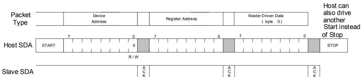
Figure 27. I 2 C Write Example
