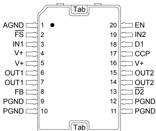
Figure 3. 33887 Pin Connections
