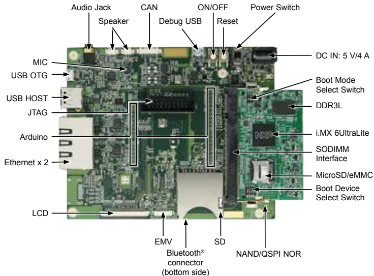
Figure 1: Main interfaces of i.MX 6UltraLite EVK
