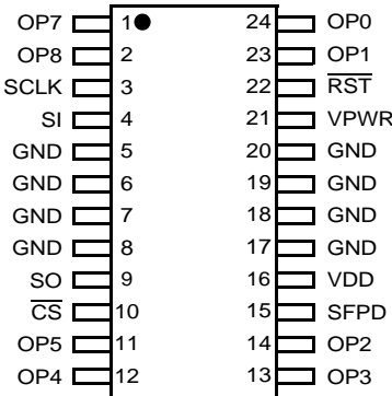
Figure 3. 33298 Pin Connections
