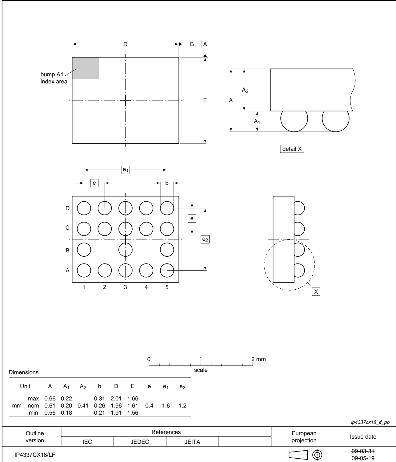
Fig 7. Package outline IP4337CX18/LF (WLCSP18)
