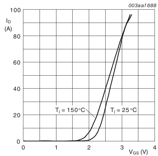
Fig 9. Transfer characteristics; drain current as a function of gate-source voltage
