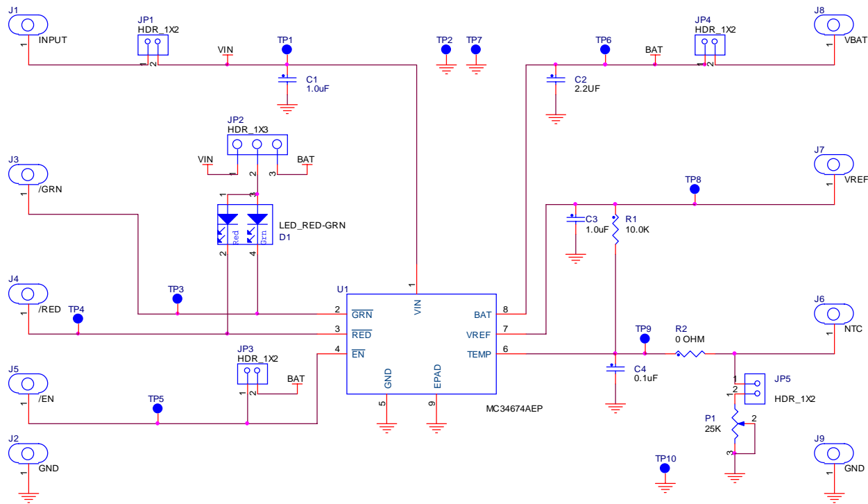
Figure 2. Schematic Circuit
