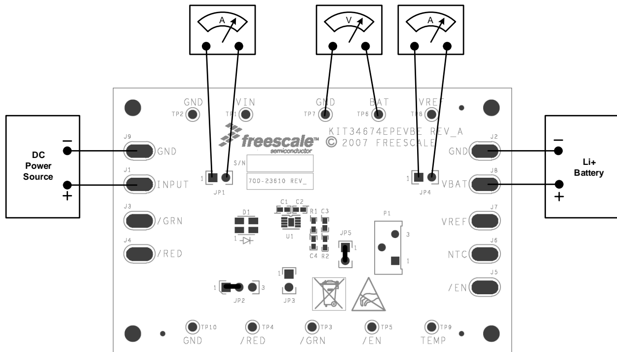
Figure 7. Test Setup
