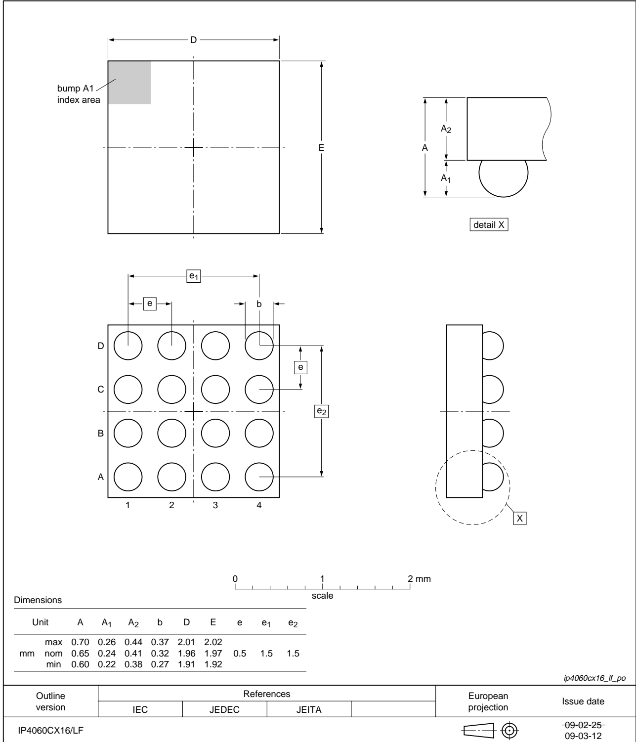
Fig 3. Package outline IP4060CX16/LF (WLCSP16)
